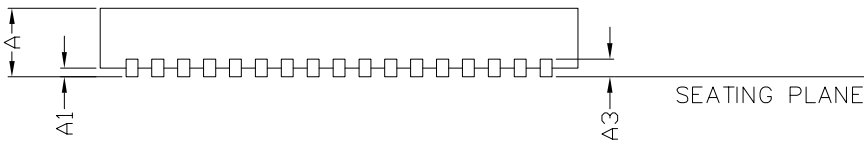
SIDE VIEW
