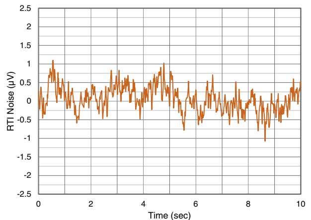
Figure 15. 0.1Hz to 10Hz RTI Voltage Noise
