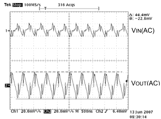
Scope Photo #4 Voltage Ripple (1.5X Mode)
